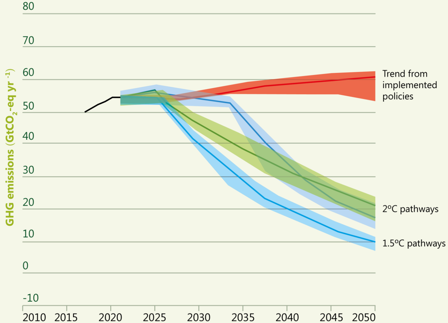
Future global greenhouse-gas emissions for Paris targets, CO 2 equivalent
